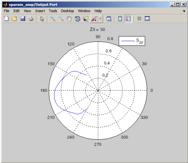
S_{22} versus Frequency for a Physical Subsystem
